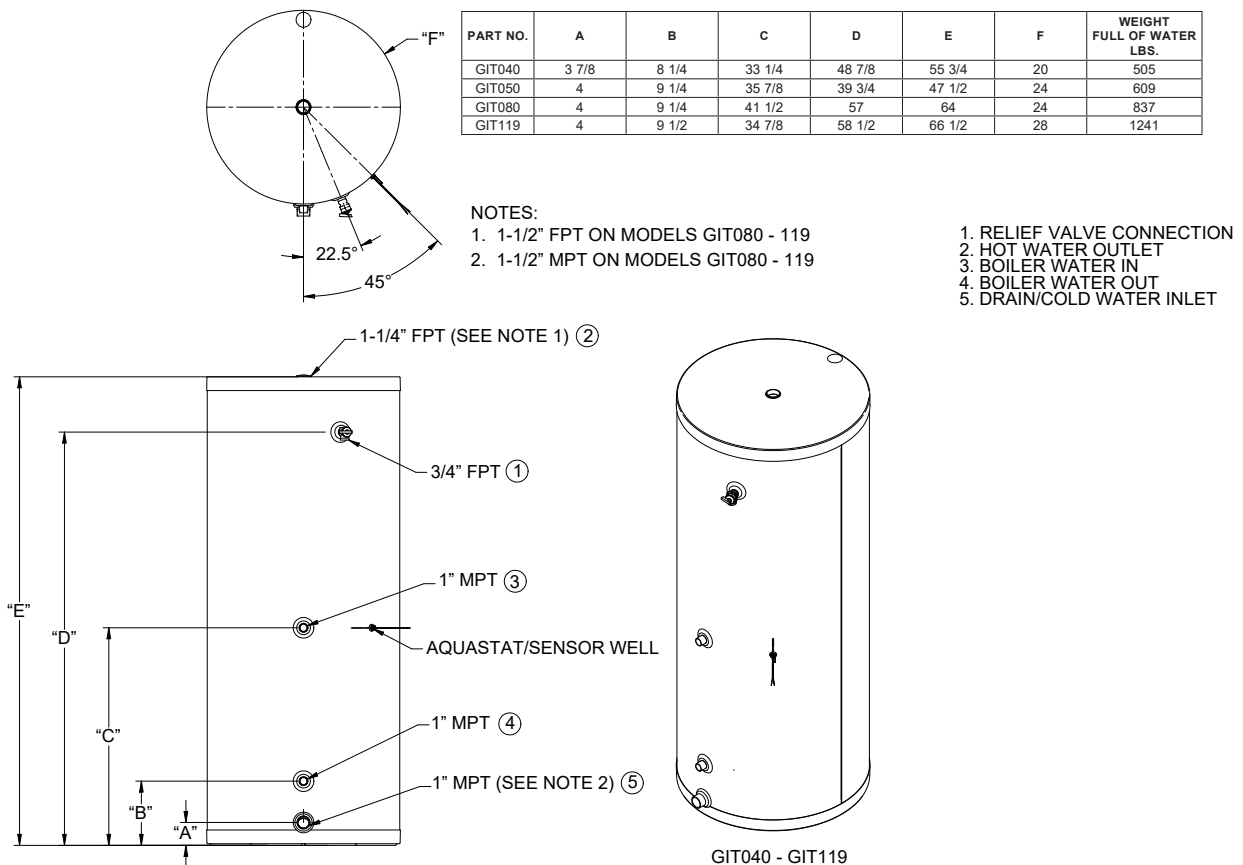
Figure 1-1 Lochinvar GIT Series Indirect Water Heater
